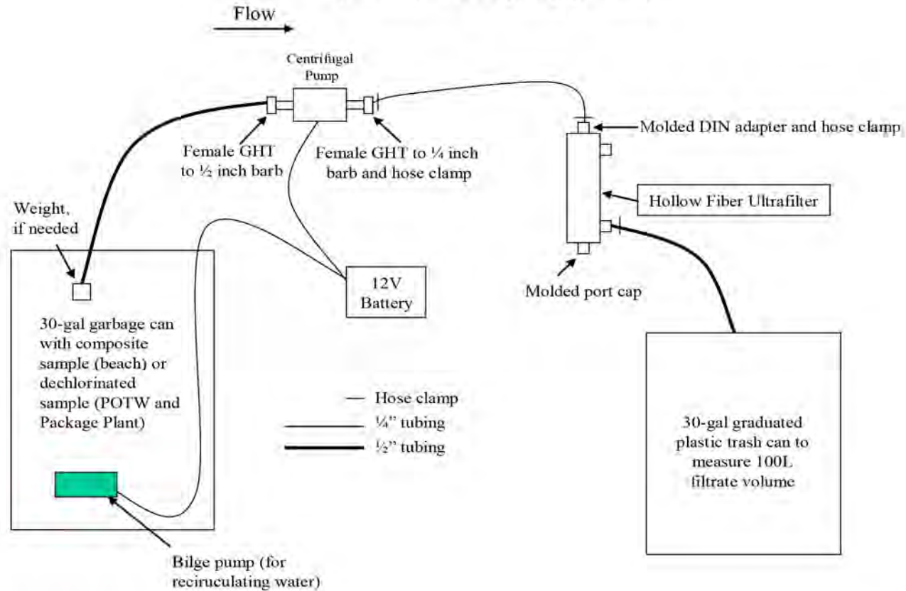
Figure C.A-2. Sampling setup at the beach, POTW, and package plant sites (there will be two identical setups, because two filters will be used).
